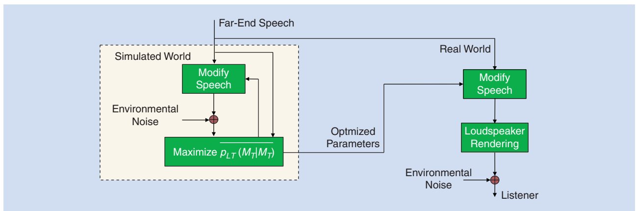
[FIG3] The intelligibility enhancement using a phoneme-level measure.
