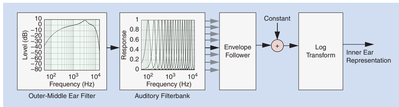
[FIG1] The basic structure of the auditory model presented in [21].
