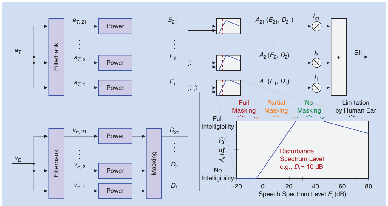
[FIG2] The computation of the SII.
