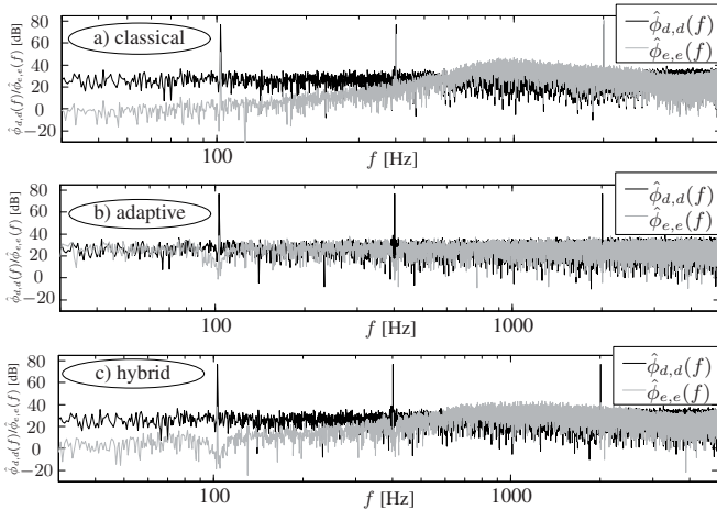
Fig. 6. Noise attenuation curves for a) the non-adaptive (classical), b) the adaptive and c) the novel hybrid feedback ANC approaches. The ambient noise signal is Gaussian white noise mixed with three sinusoidal signals at f_0 = 103 , f_1 = 401 and f_2 = 2005 Hz.
