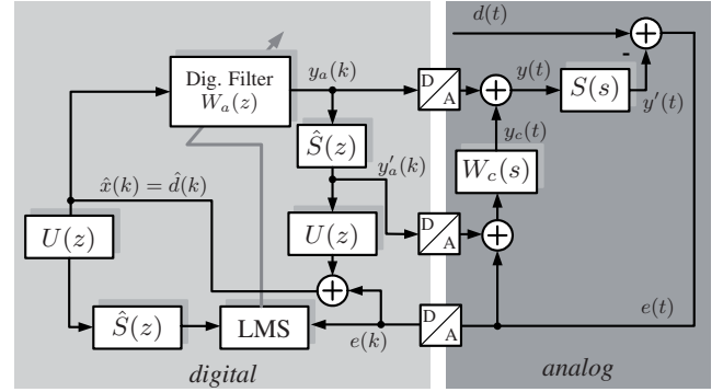
Fig. 5. Mixed analog-digital realization of proposed hybrid feedback ANC approach.
