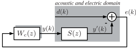
Fig. 2. Model for a classical feedback ANC system.
