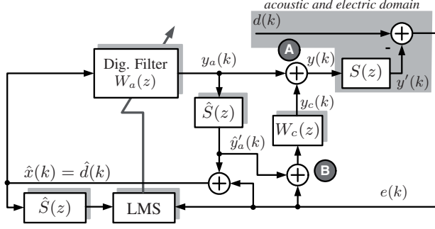
Fig. 4. The novel hybrid feedback ANC system based on the FxLMS approach.
