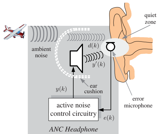
Fig. 1. Hardware setup of a broadband feedback ANC headset.
