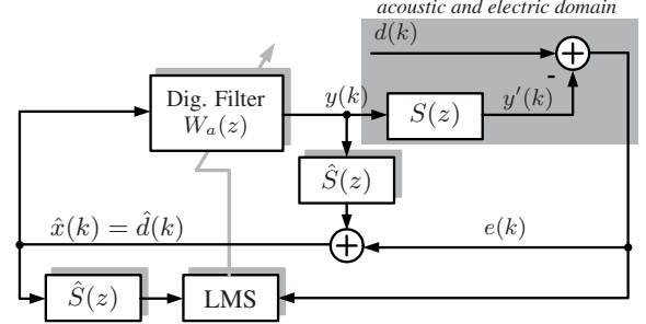
Fig. 3. Model for an adaptive feedback ANC system involving the FxLMS approach.
